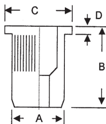
LARGE FLANGE
